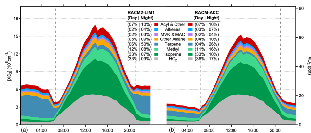
Figure 5. Modeled \text{XO}_2 composition from RACM2-LIM1 (a) and RACM-ACC (b). Colors represent peroxy radicals derived from the listed VOCs and numbers represent the percentage contribution of each species to the total concentration of \text{XO}_2 during the day (06:30 to 21:00) and at night (21:00 to 06:30), respectively.
