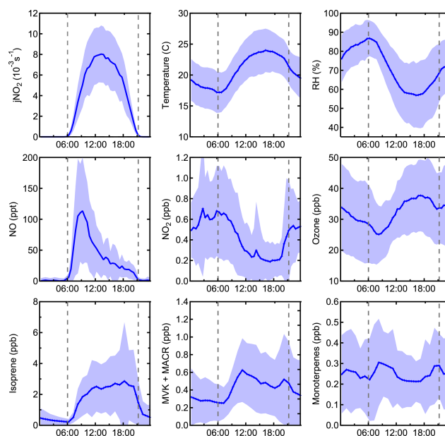
Figure 2. Campaign average measurements of j\text{NO}_2 , temperature, relative humidity, NO, \text{NO}_2 , \text{O}_3 , isoprene, methyl vinyl ketone and methacrolein, and monoterpenes. Shaded areas represent the 1\sigma variability.
